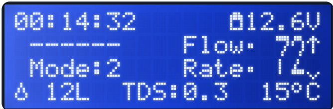
A long press swaps modes — here the FlowOne has jumped to Mode 2 and its higher flow rate.
